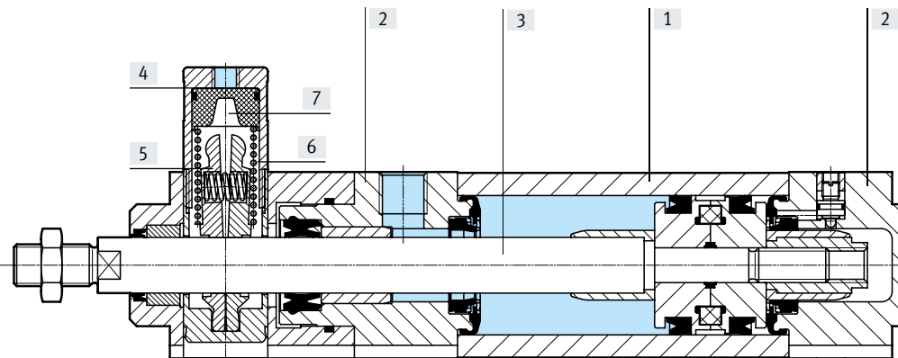
Standards-based cylinder
