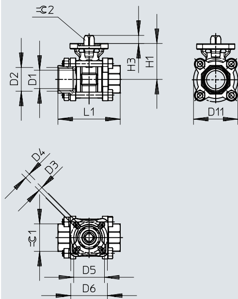
Dimensions – Ball valves VZBE, 2-way, with pipe thread
