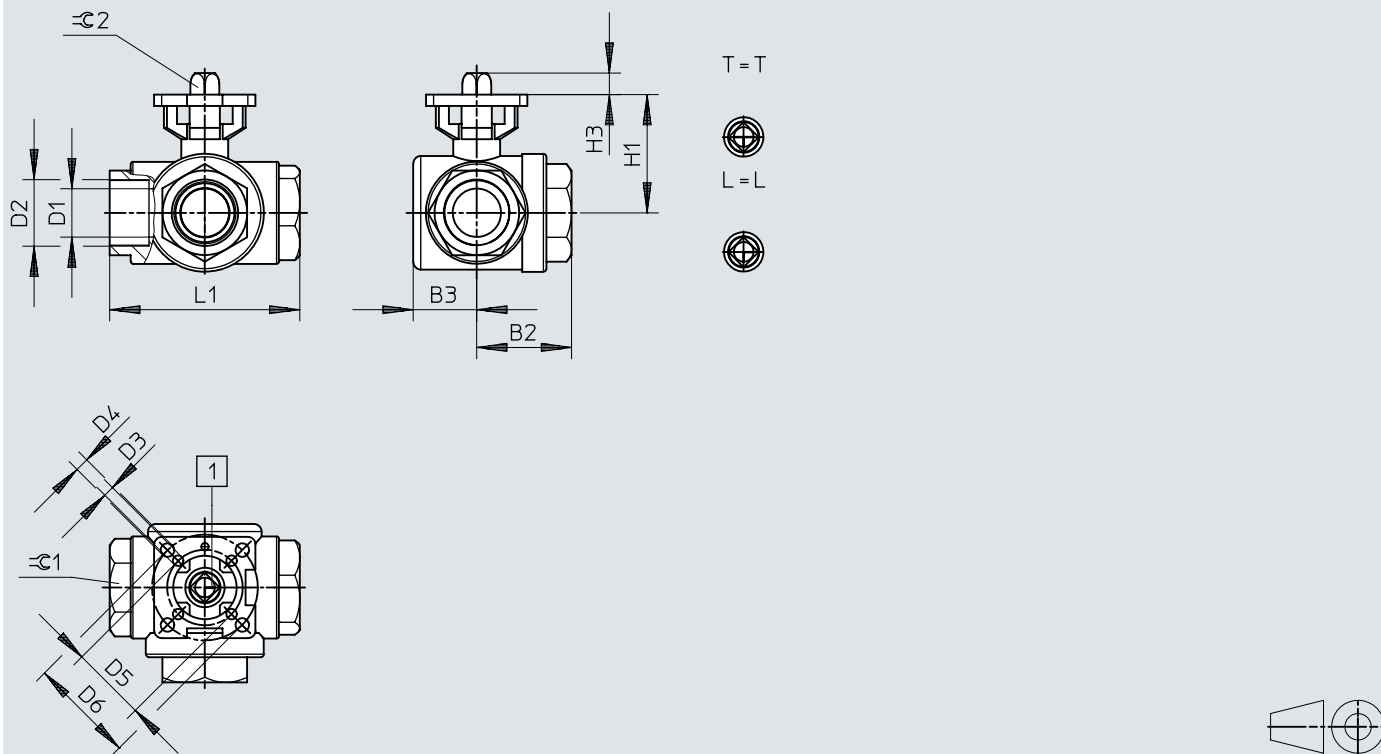
Dimensions – Ball valves VZBE, 3-way, with pipe thread
