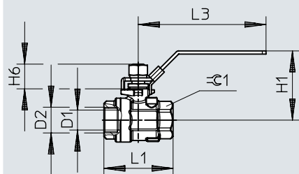
Dimensions – Ball valves VZBE, 2-way, with hand lever and pipe thread
