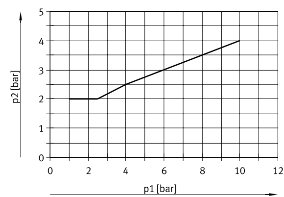
For 5/2-way valves, single solenoid
