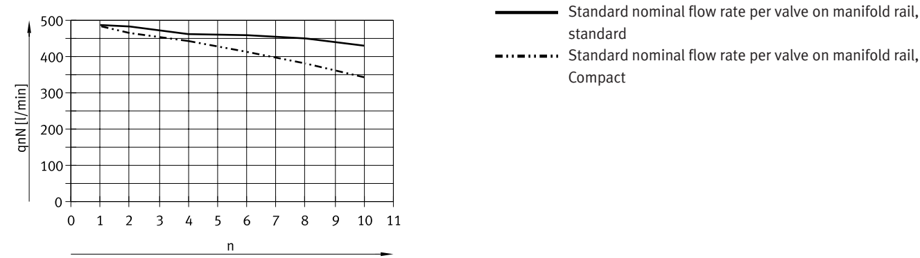
For 5/2-way valves, flow direction 1 → 4
