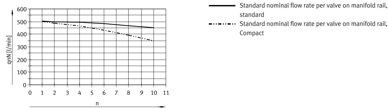
For 5/2-way valves, flow direction 1 → 2
