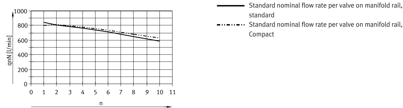
For 5/2-way valves, flow direction 1 → 4
