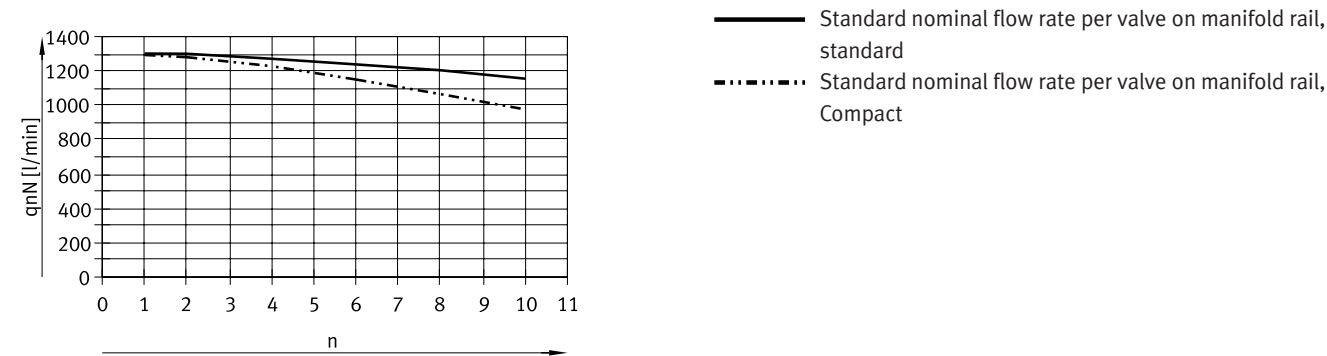
For 5/2-way valves, flow direction 1 → 2
