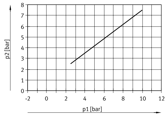
For 5/2-way valves, double solenoid
