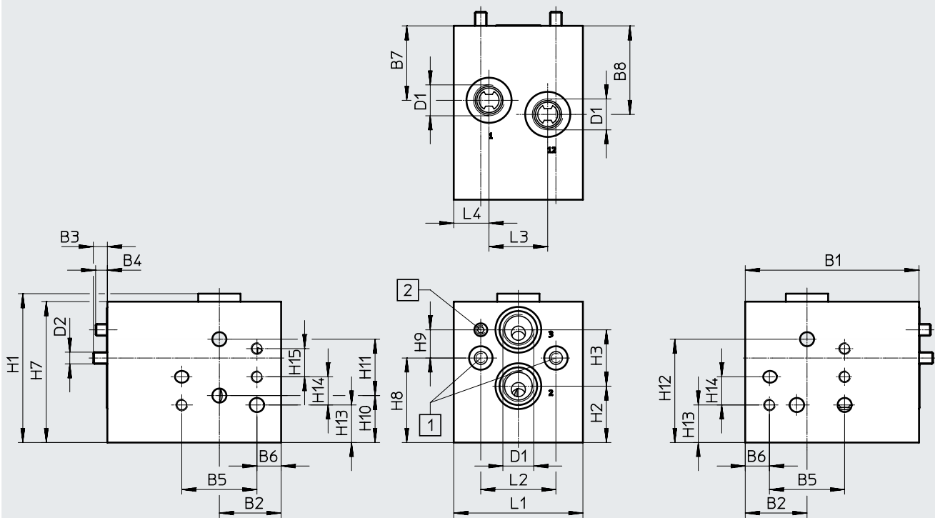
[1] 内六角螺丝 M5x70 [2] 螺纹销 M5x10
