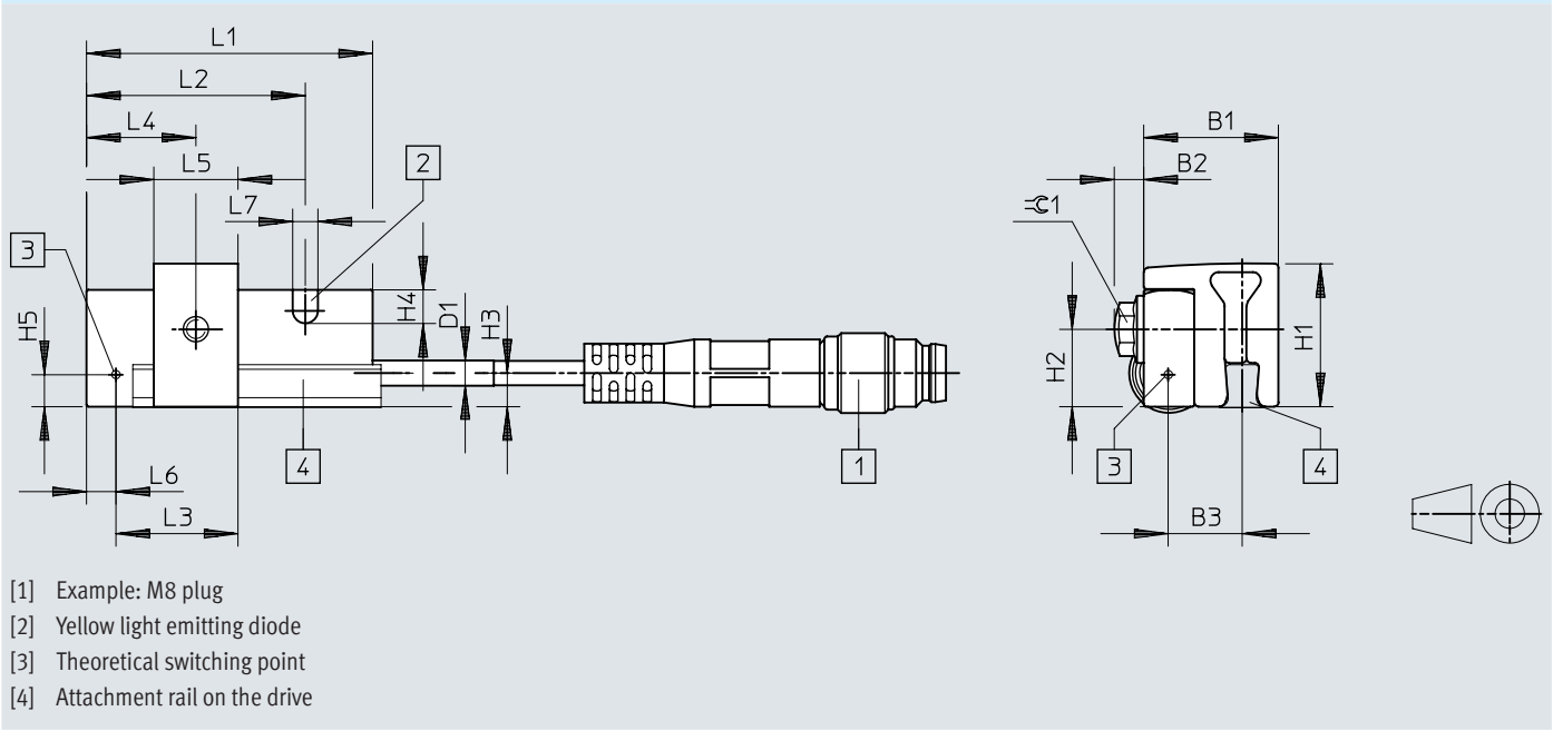
Dimensions – SMT-C1
