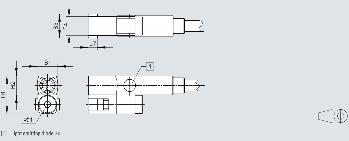
Dimensions – SMT-8-G
