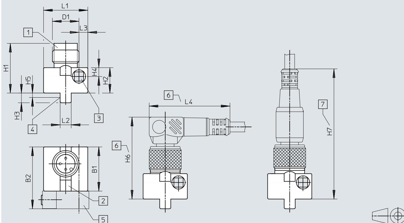
Dimensions – SMT0-8E-...-M12-LED-24 – Plug M12x1
