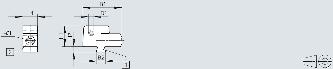
Dimensions – Mounting kit SMB-8E
