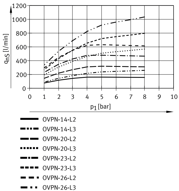
Suction rate q_{nS} (against atmosphere) as a function of operating pressure p_1
