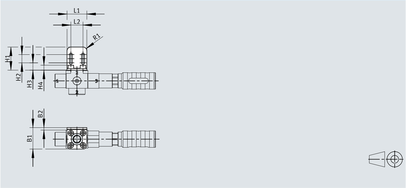
Dimensions – OVPN-14 (OVPN-14-L...-PG14-G12-UA)
