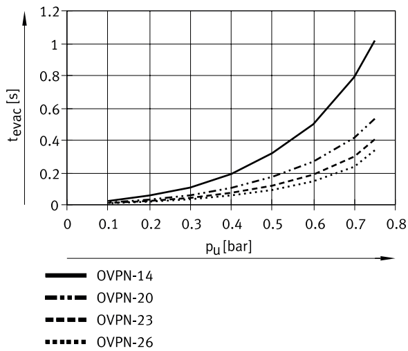
Evacuation time t as a function of vacuum p_u for 1 l volume at 6 bar operating pressure
