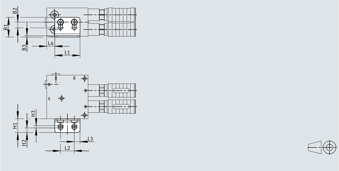
Dimensions – OVPN-20/23/26 (OVPN-...-L...-PG14-G34-UA)
