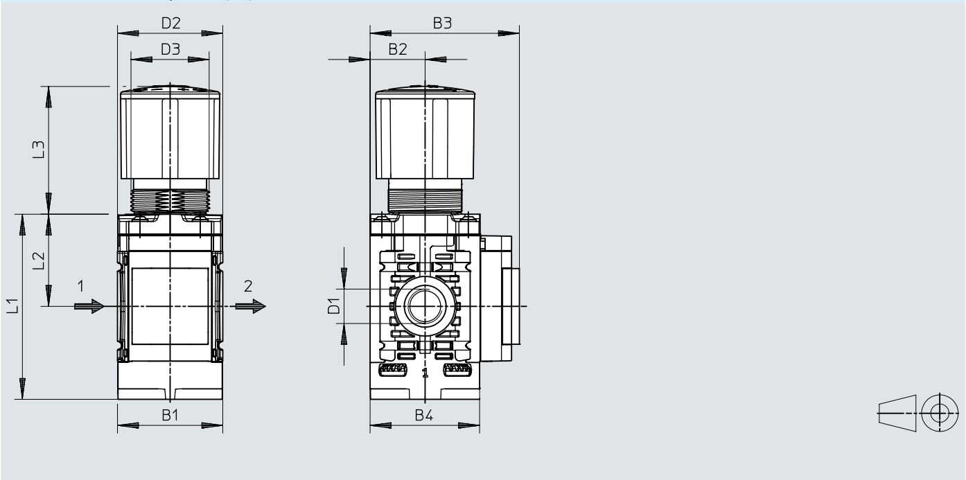
Dimensions – MS4-LR with pressure gauge
