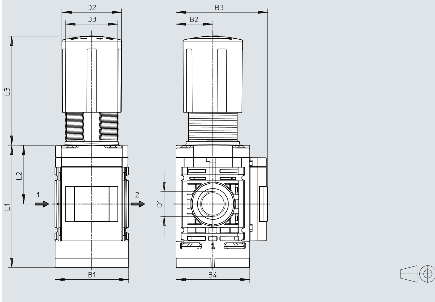
Dimensions – MS6-LR with pressure gauge
