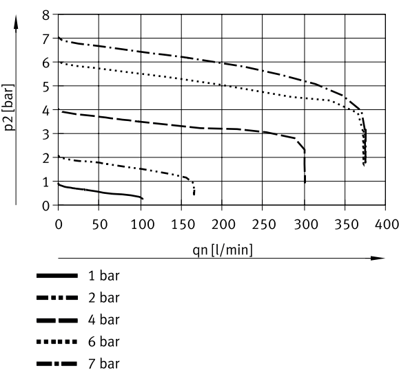
Standard flow rate q_n as a function of output pressure p_2 ( p_1 = 10 \text{ bar} ) – MS2-LR-M5-B
