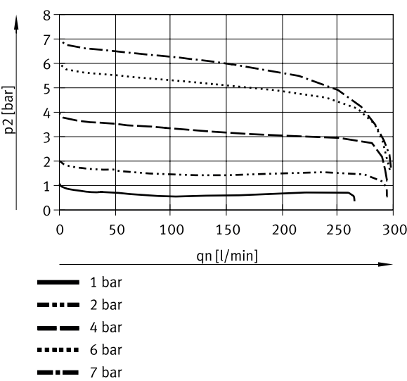
Standard flow rate q_n as a function of output pressure p_2 ( p_1 = 8 \text{ bar} ) – MS2-LR-QS6-B
