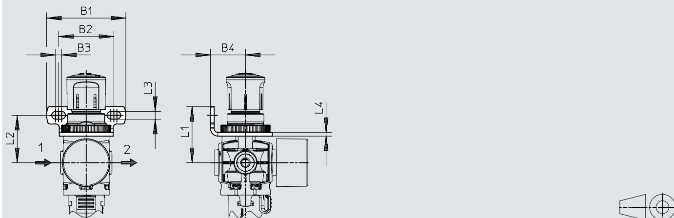
Dimensions – Mounting bracket MS...-WR-B
