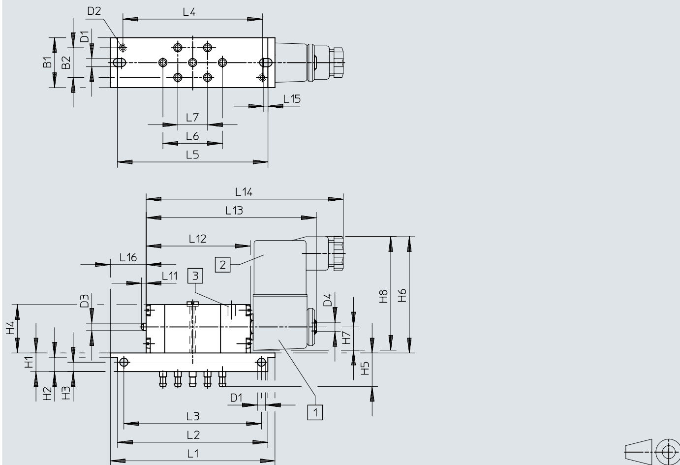
Dimensions – MFH-5-PK-3(-L)
