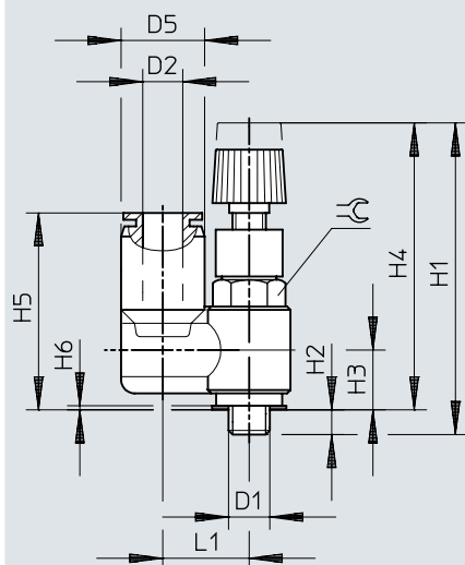
Dimensions – Outlet at the top, pneumatic connection 1: M5
