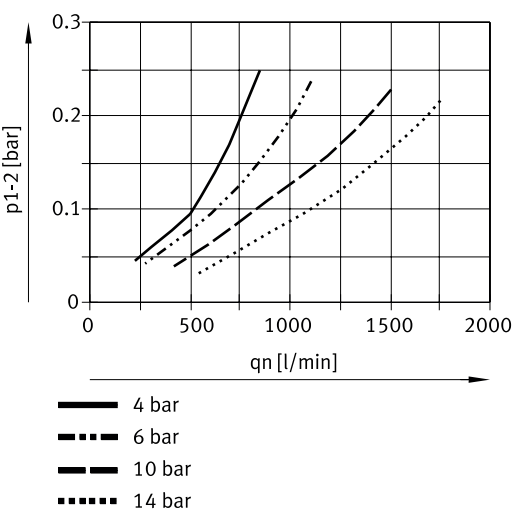
Standard flow rate q_n as a function of differential pressure \Delta p_{1-2} (LFMA-1/2-D-MIDI)
