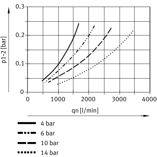
Standard flow rate q_n as a function of differential pressure \Delta p_{1-2} (LFMA-1-D-MAXI)
