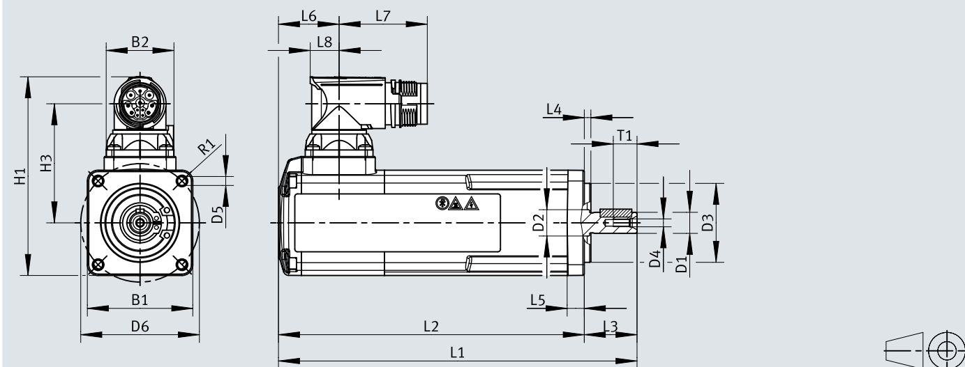
Dimensions – EMMT-EC-40
