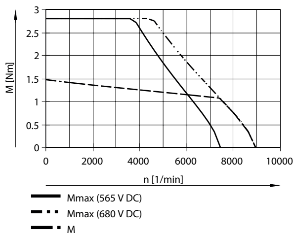
Torque M as a function of rotational speed n for EMMT-AS-80-S-HS, short, high voltage, without/with brake
