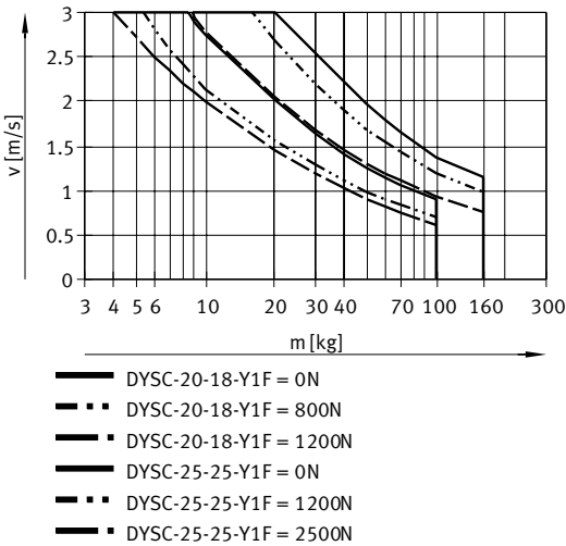
Impact velocity v as a function of mass m – DYSC-20/25
