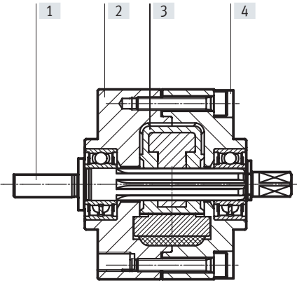
DRVS-6/8
