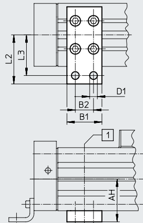
Piston Ø 32 ... 63
