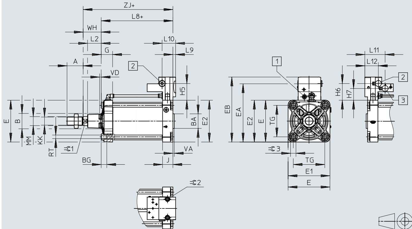
Dimensions – Variant DFPI-...-ND2P-E-NB3VM12
