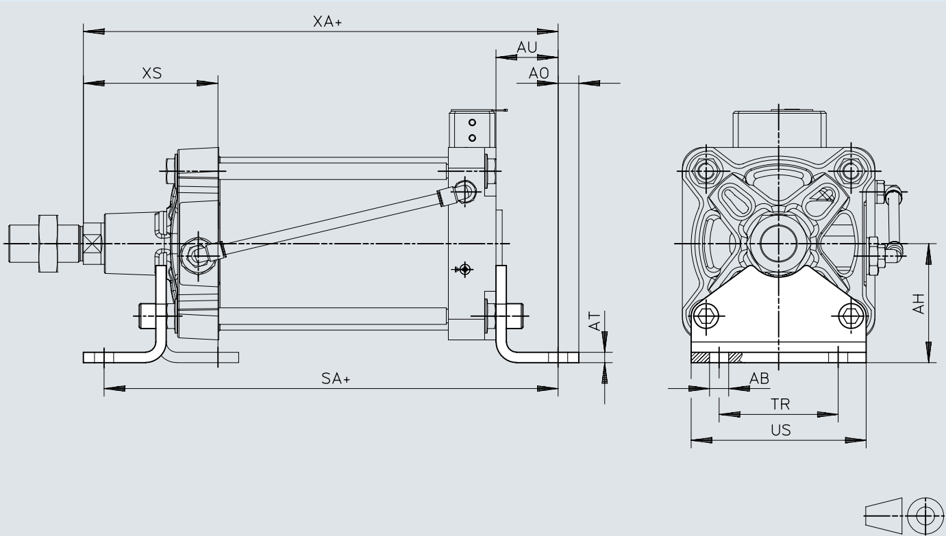
Dimensions – Foot mounting HNG, for Ø 160, 200
