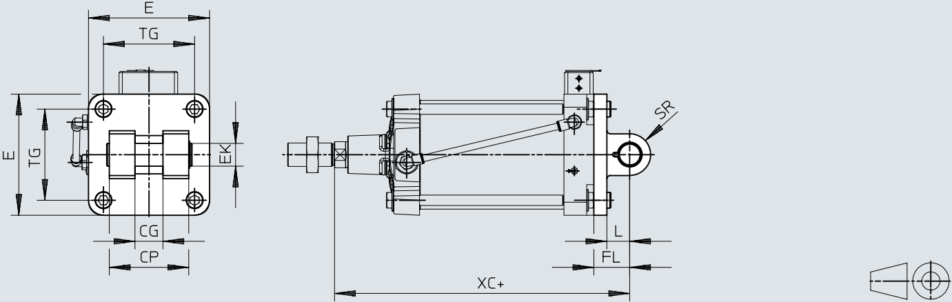
Dimensions – Swivel flange SNG
