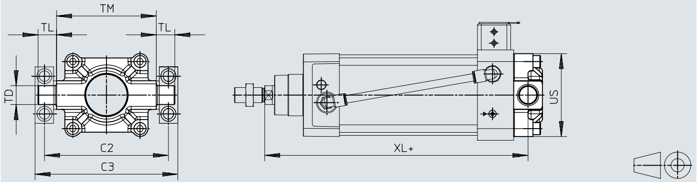
Dimensions – Trunnion flange ZNCF/CRZNG
