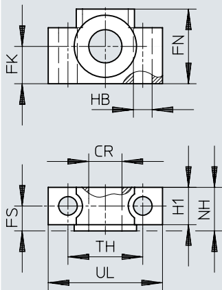
Dimensions – Trunnion support CRLNZG
