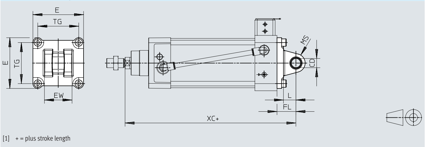
Dimensions – Swivel flange SNCL
