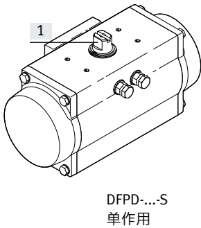
[1] The position of the shaft in the delivery condition
