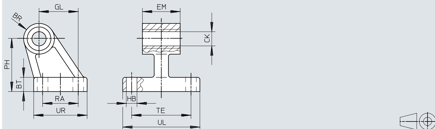
Dimensions – Clevis foot CRLNG
