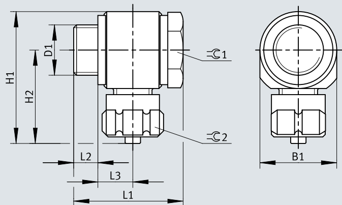
Dimensions – Elbow quick connector LCK/LCK-...-KU
