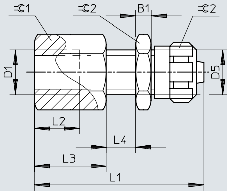
Dimensions – Bulkhead quick connector QCK
