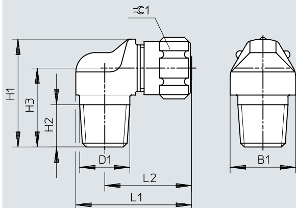
Dimensions – Elbow quick connector GCK-...-KU
