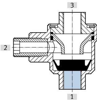
[SE] Quick exhaust valve
