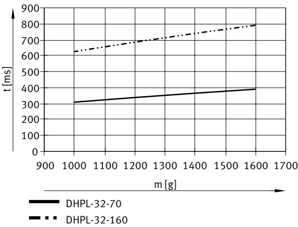
Opening and closing times as a function of gripper finger mass – DHPL-32
