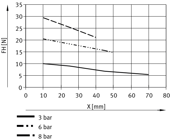
Gripping force F per gripper jaw as a function of operating pressure and lever arm x – External gripping (closing), double-acting – DHPL-10-20-...-A
