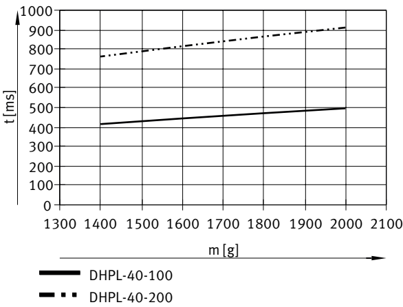
Opening and closing times as a function of gripper finger mass – DHPL-40
