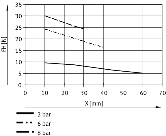
Gripping force F per gripper jaw as a function of operating pressure and lever arm x – External gripping (closing), double-acting – DHPL-10-60-...-A
