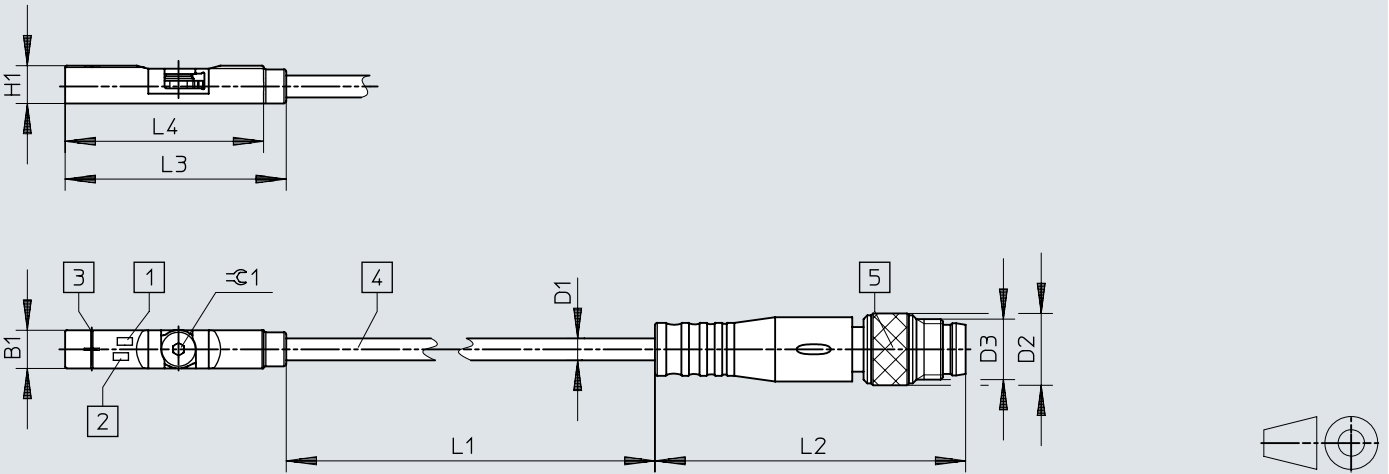
Dimensions – With BG M8D plug
