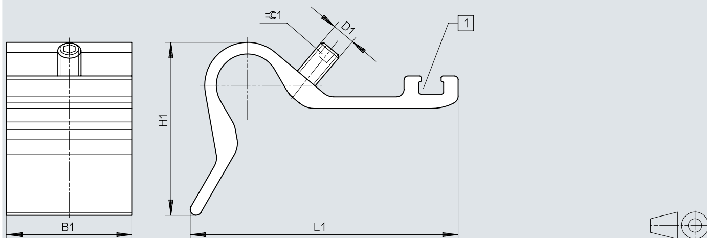
Dimensions – Sensor bracket DASP-M4-...-A
