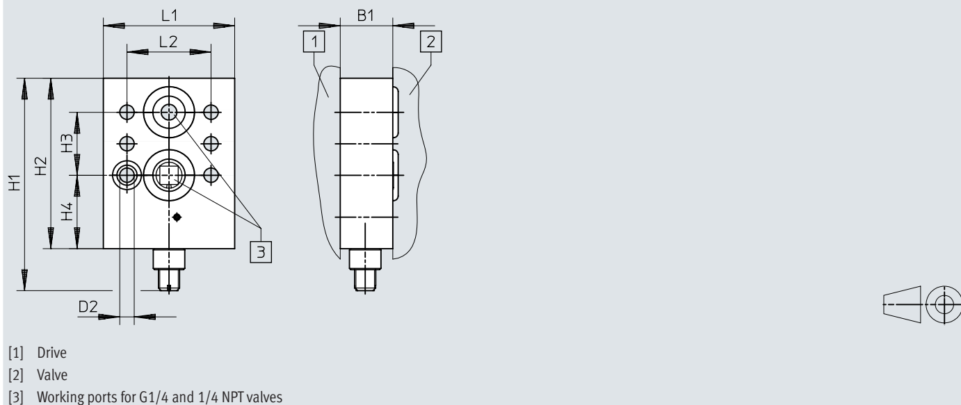
Dimensions – Throttle plate VABF-S7-F1B5P1-F for single-acting drives
