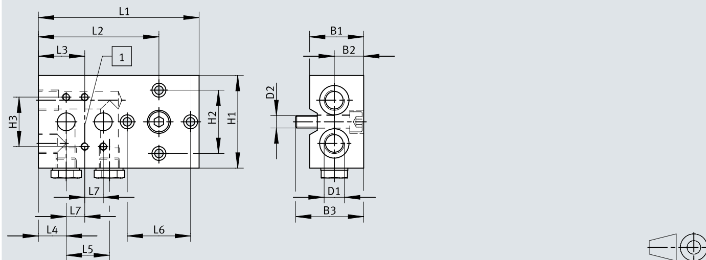
Dimensions – Sub-base VABS-S7-S-G14
