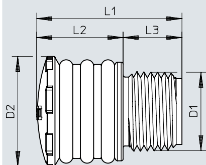
Dimensions – Exhaust protection VABD-D3-SN-N12
