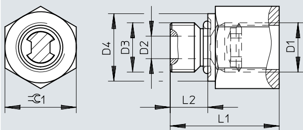
Dimensions – Adapter with filter NPFV-AF-...
