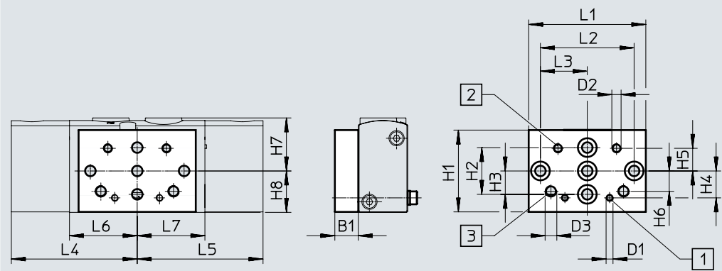
[1] Mounting hole for size 20 [2] Mounting hole for size 25 [3] Mounting hole for size 30
