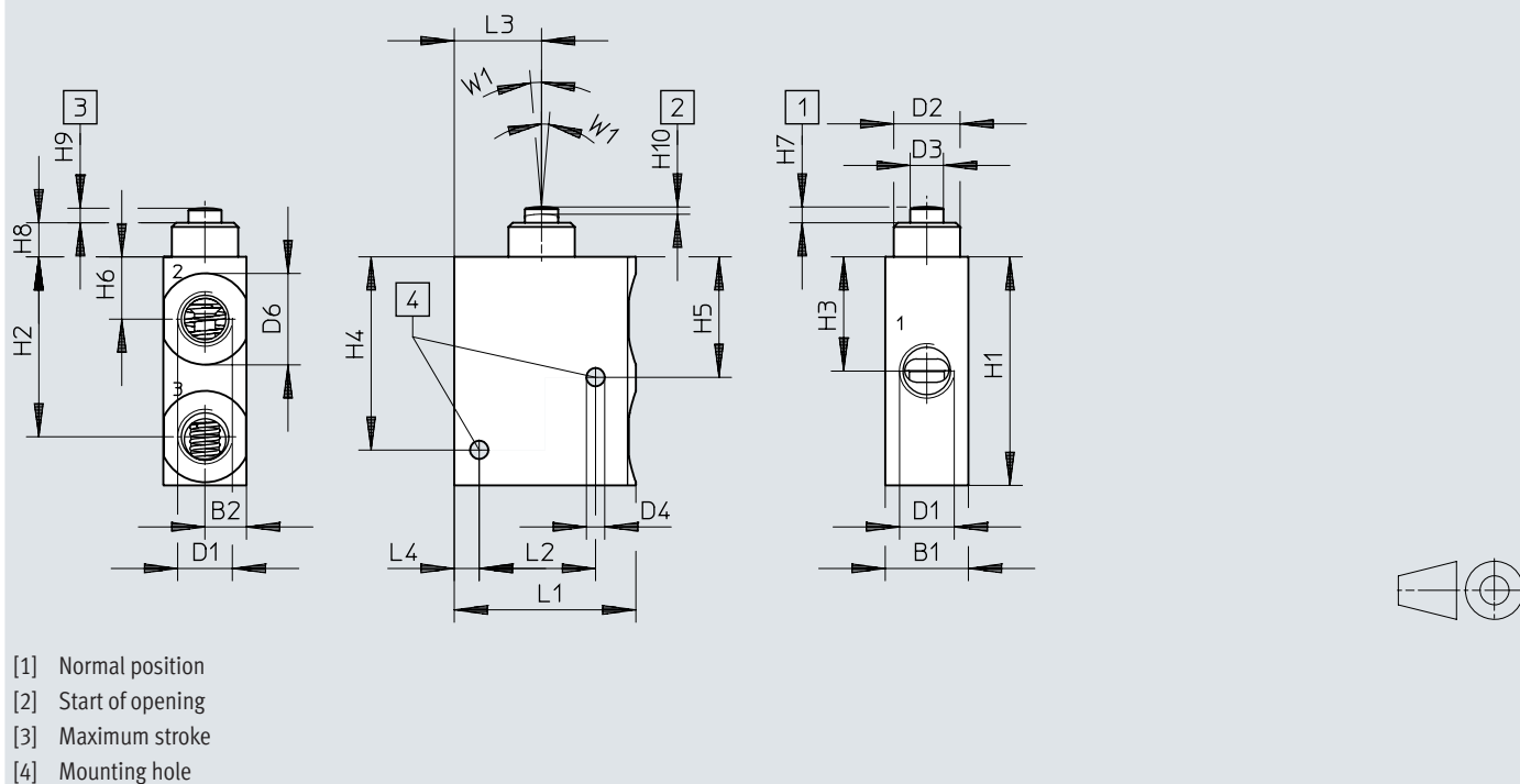
Dimensions – Stem actuated 3/2-way valve
