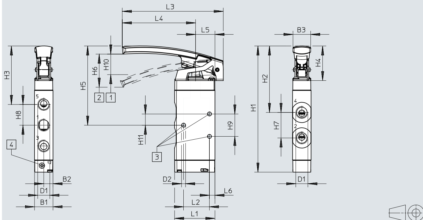
Dimensions – 5/2-way valve, finger lever valve
