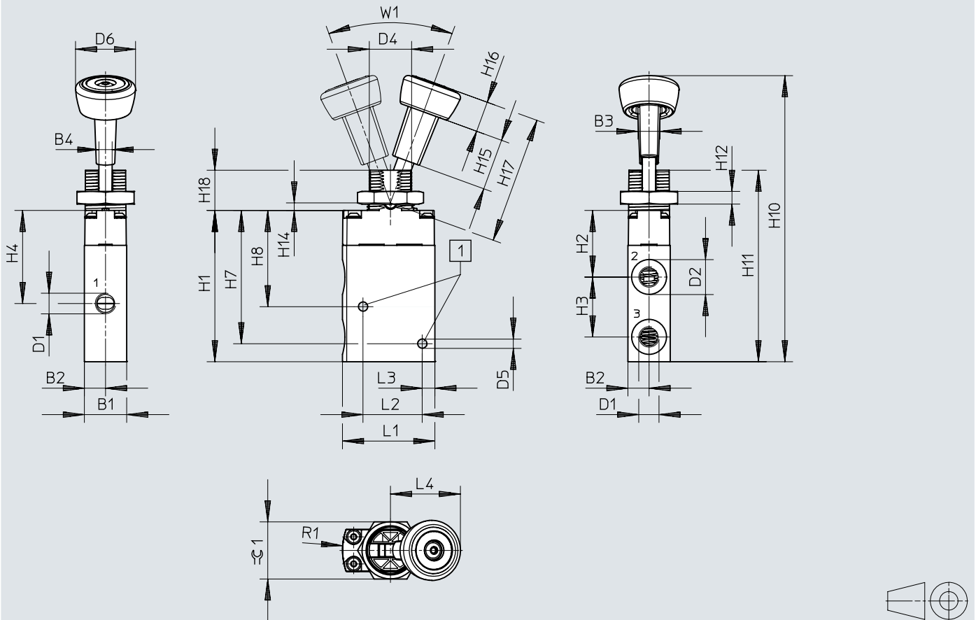
Dimensions – 3/2-way valve, toggle lever valve
