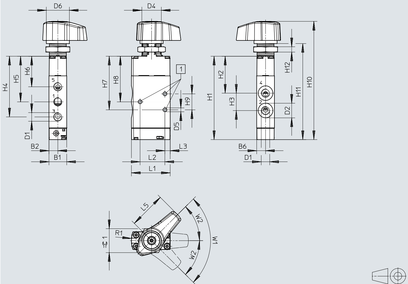
Dimensions – 5/2- and 5/3-way valve, selector valve
