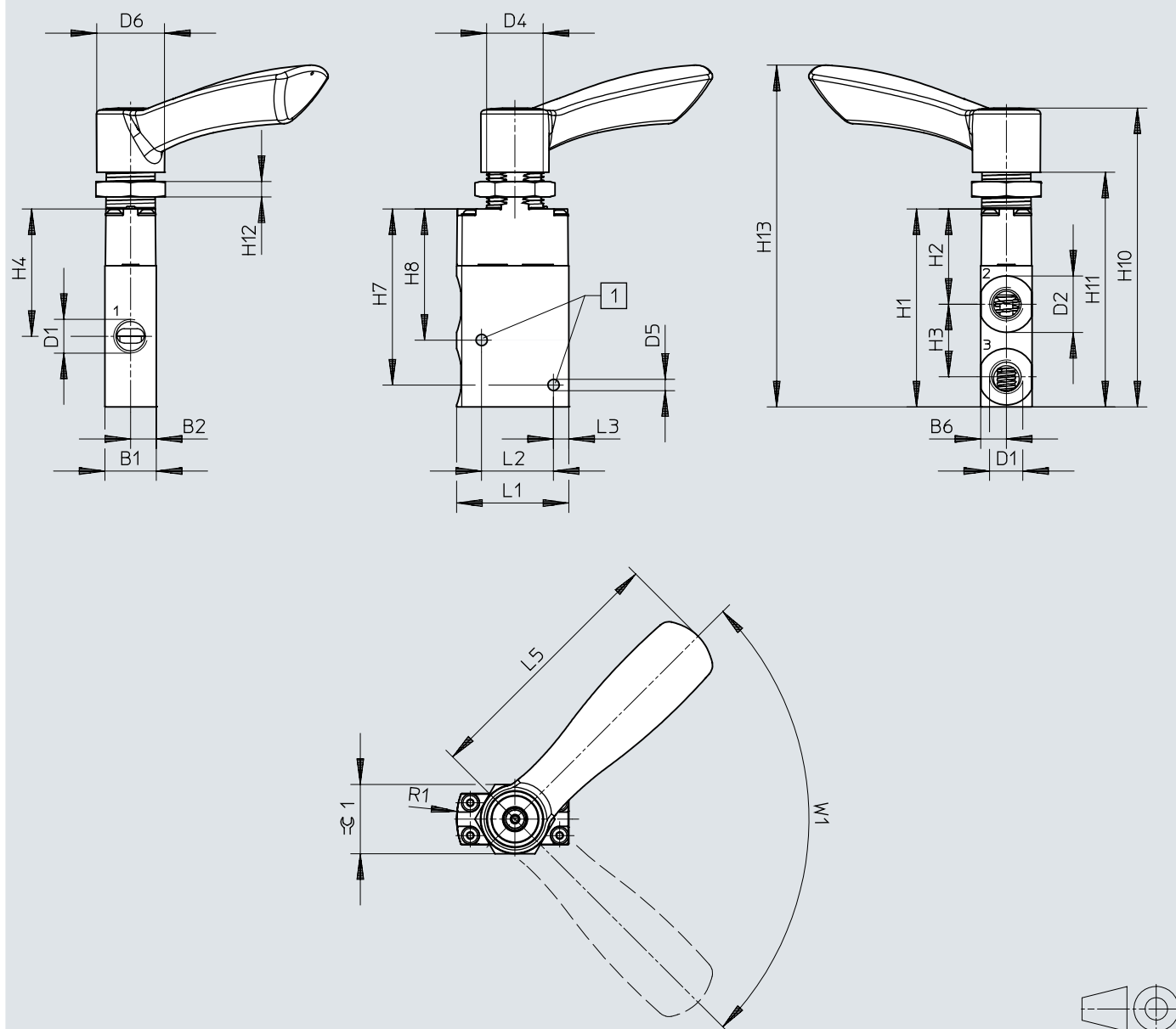
Dimensions – 3/2-way valve, hand lever valve
