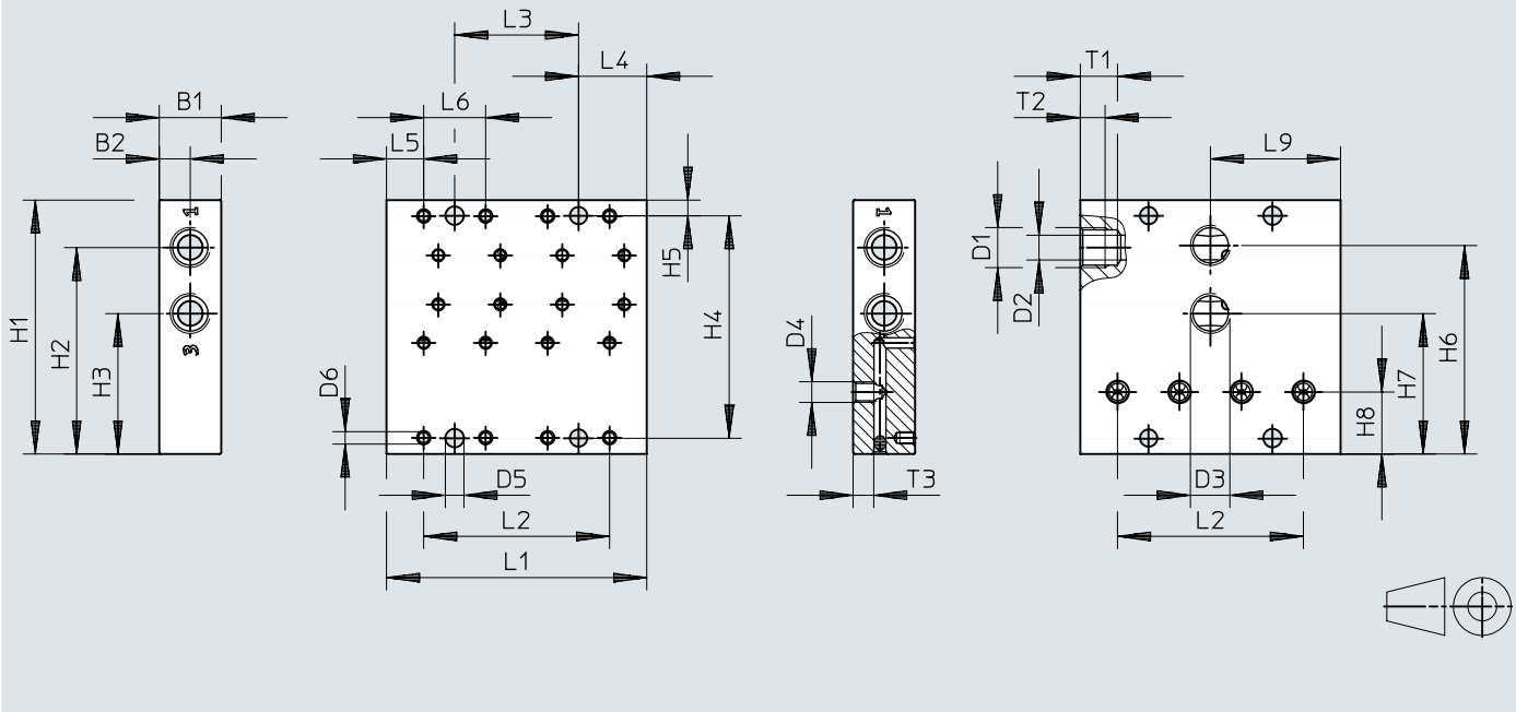
Dimensions – Manifold rail, connection direction underneath
