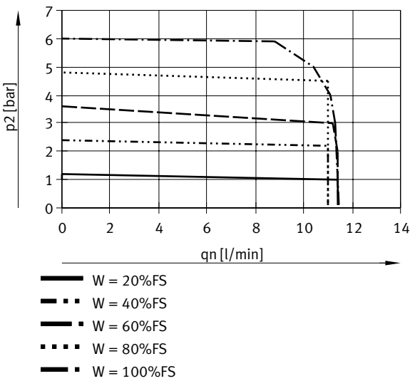
VEAA-...-D9-..., output pressure 2 (pressure regulation range) 0.03 ... 6, flow rate qn from 1 -> 2 depending on output pressure p2
