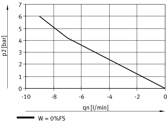
VEAA-...-D9-..., output pressure 2 (pressure regulation range) 0.03 ... 6, flow rate qn from 2 -> 3 depending on output pressure p2
