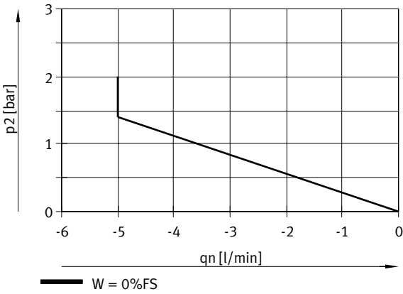
VEAA-...-D2-..., output pressure 2 (pressure regulation range) 0.01 ... , flow rate qn from 2 -> 3 depending on output pressure p2
