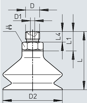
Dimensions – Dimensions – Suction cup VASB-...-SI-B, protective bellows
