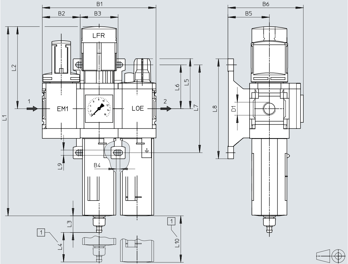
[1] Installation dimension
