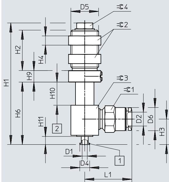
Dimensions – ESH-HDL, push-in connector QS, size 2
