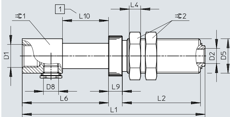
Dimensions – ESH-HCL, threaded connection G, size 6
