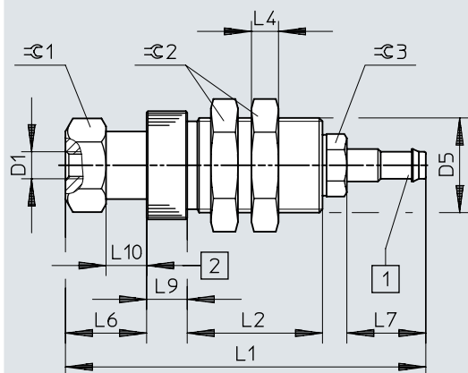
Dimensions – ESH-HC, barbed connector PK, size 3/4
