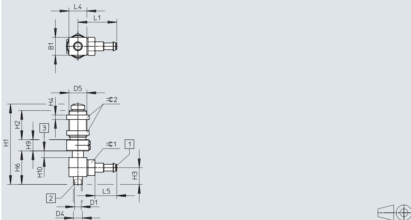
Dimensions – ESH-HD, barbed connector PK, size 1
