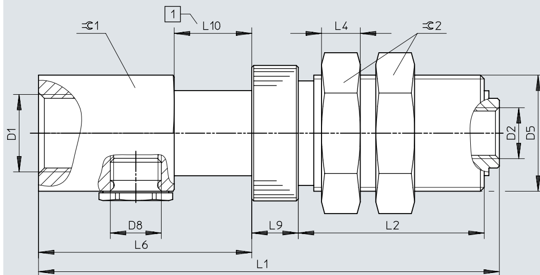
Dimensions – ESH-HC, threaded connection G, size 6
