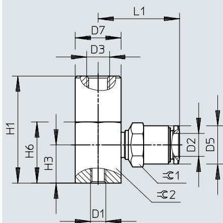
Dimensions – ESH-HB, push-in connector QS, size 3
