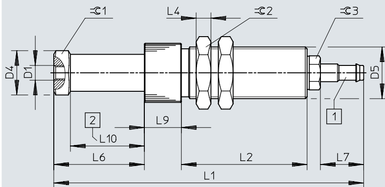
Dimensions – ESH-HCL, barbed connector PK, size 3/4
