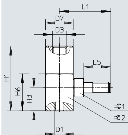
Dimensions – ESH-HB, barbed connector PK, size 3
