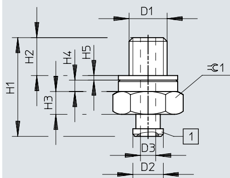
Dimensions – ESH-HE, G and M thread, size 2
