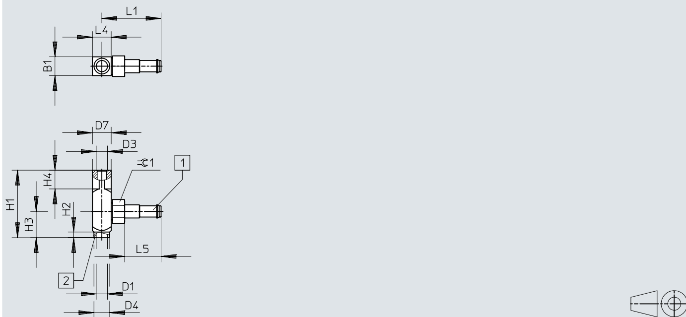
Dimensions – ESH-HB, barbed connector PK, size 1
