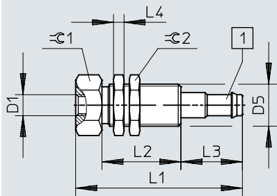
[1] Barbed connector PK-4 for plastic tubing
