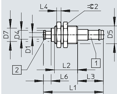
Dimensions – ESH-HA, barbed connector PK, size 2
