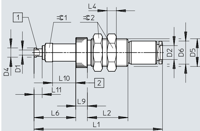
Dimensions – ESH-HCL, push-in connector QS, size 2
