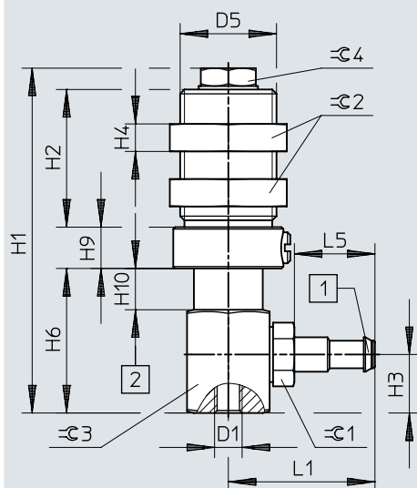
Dimensions – ESH-HD, barbed connector PK, size 3/4
