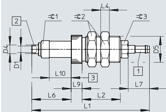
Dimensions – ESH-HCL, barbed connector PK, size 1
