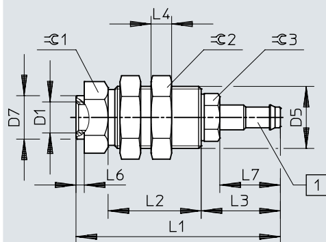
Dimensions – ESH-HA, barbed connector PK, size 4
