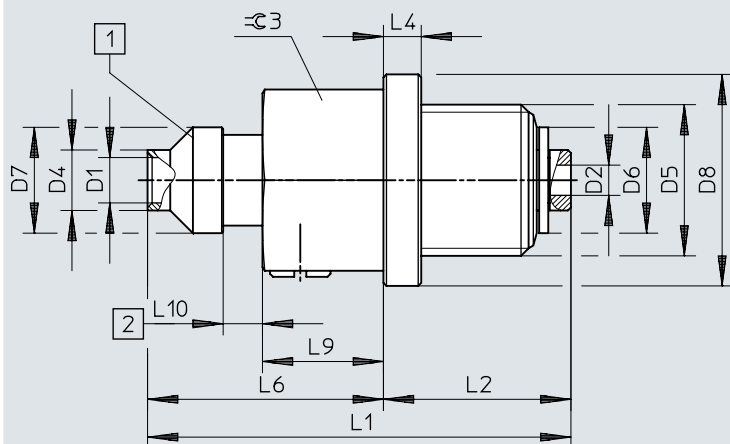
Dimensions – ESH-HF, M thread, size 1
