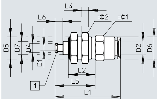
Dimensions – ESH-HA, push-in connector QS, size 2
