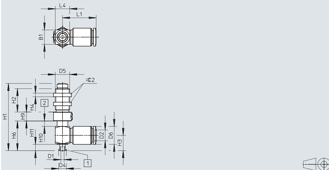
Dimensions – ESH-HD, push-in connector QS, size 2
