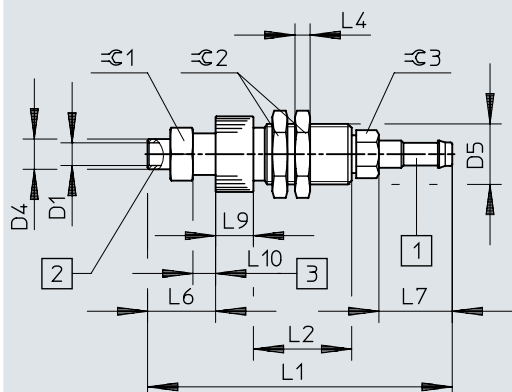
Dimensions – ESH-HC, barbed connector PK, size 1
