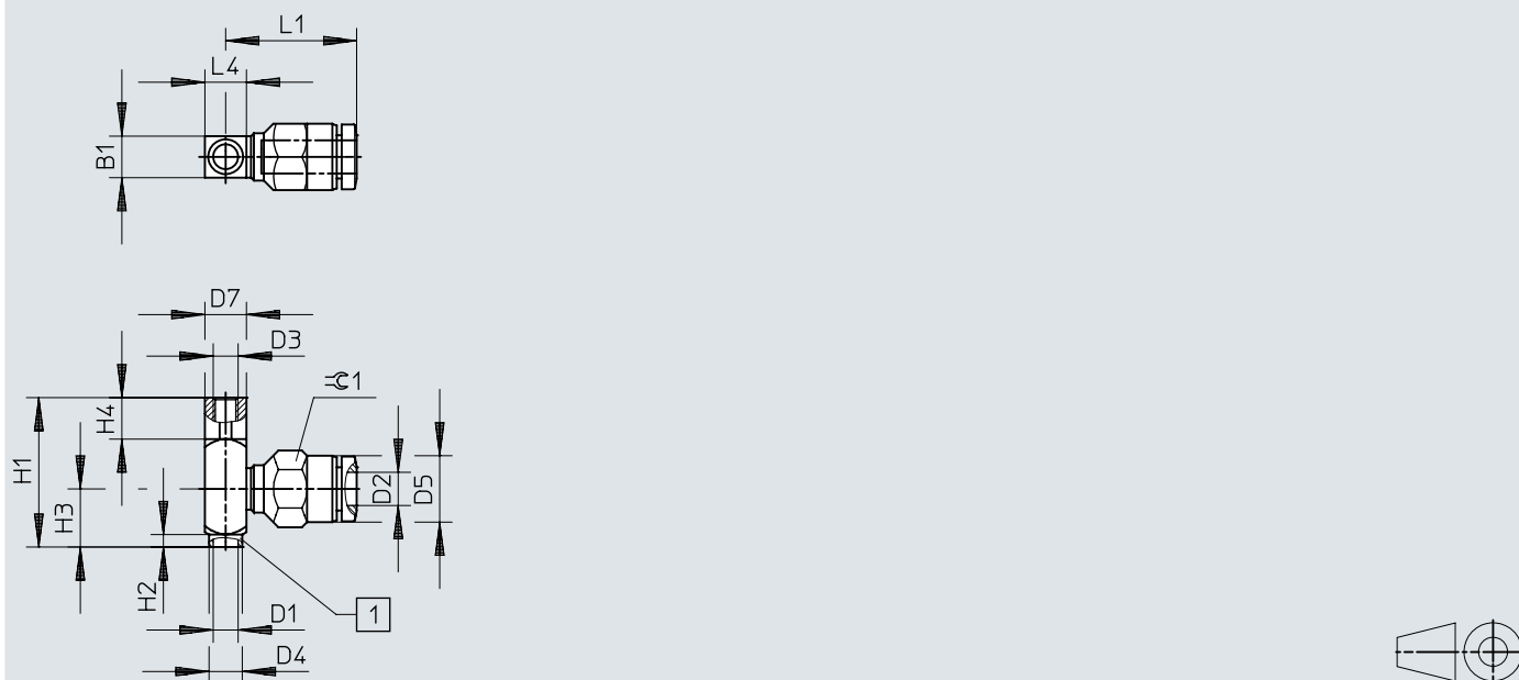
Dimensions – ESH-HB, push-in connector QS, size 1
