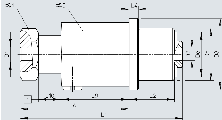
Dimensions – ESH-HF, M thread, size 3
