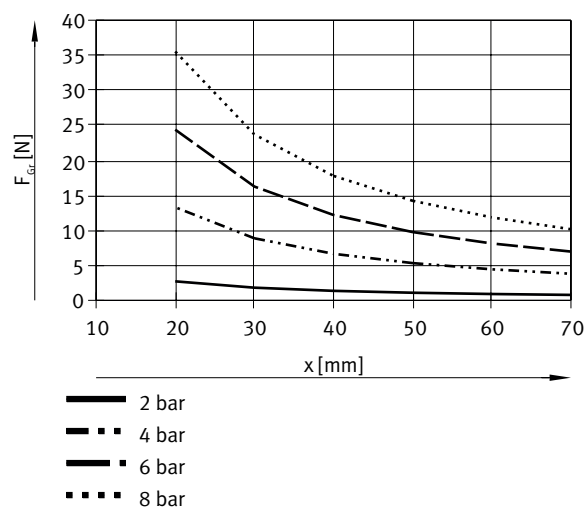
Gripping force F per gripper jaw as a function of operating pressure and lever arm x – External gripping (closing), single-acting – DHRC-16-A-S-NO
