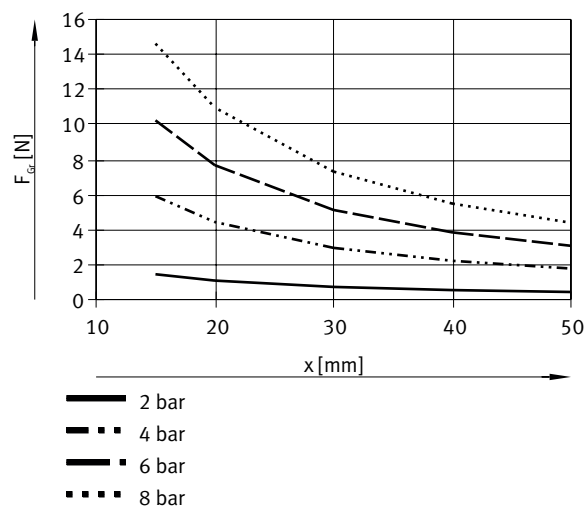
Gripping force F per gripper jaw as a function of operating pressure and lever arm x – External gripping (closing), single-acting – DHRC-10-A-S-NO
