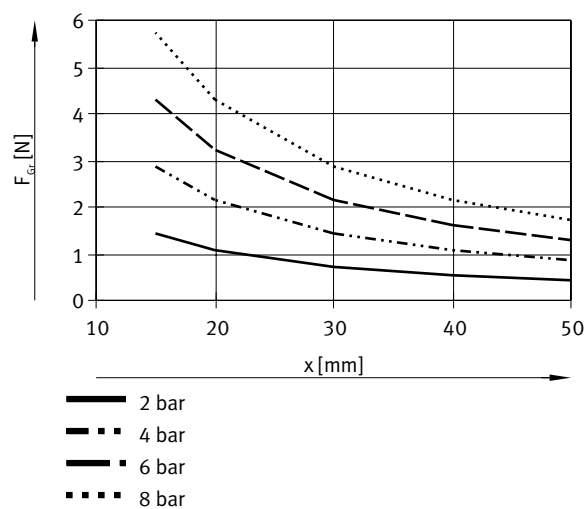
Gripping force F per gripper jaw as a function of operating pressure and lever arm x – Internal gripping (opening), double-acting – DHRC-6-A
