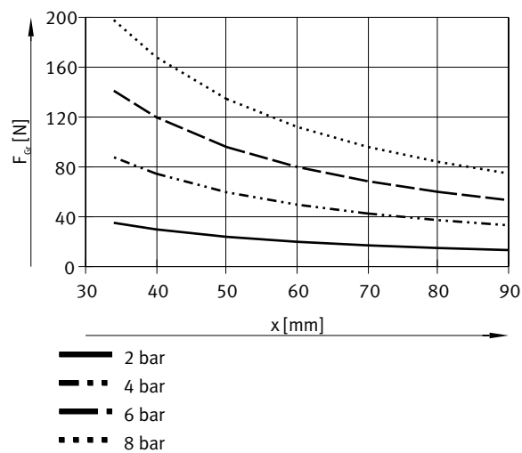
Gripping force F per gripper jaw as a function of operating pressure and lever arm x – External gripping (closing), single-acting – DHRC-32-A-S-NO
