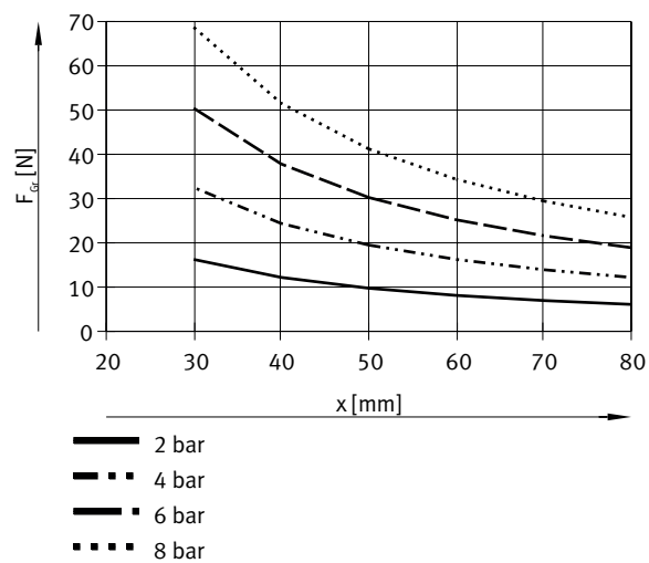
Gripping force F per gripper jaw as a function of operating pressure and lever arm x – Internal gripping (opening), double-acting – DHRC-20-A
