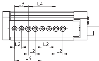
DGSL-10-40 ... 100
