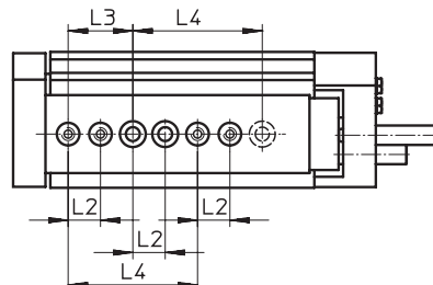
DGSL-10-40 ... 100
