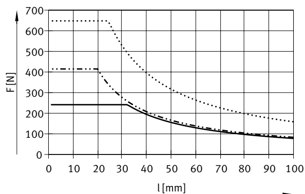
DGRC-32 ... 50, stroke 45 ... 50 mm
