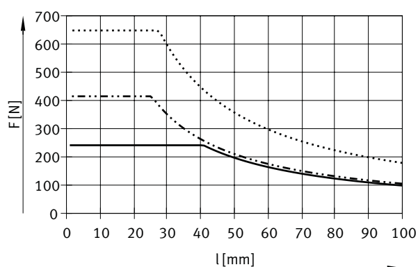
DGRC-32 ... 50, stroke 85 ... 100 mm
