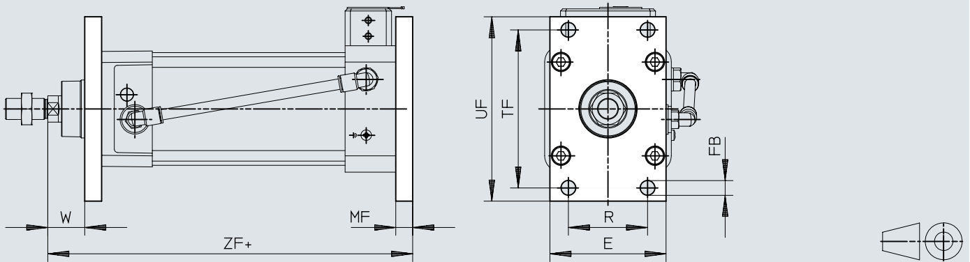
Dimensions – Flange mounting FNC/CRFNG
