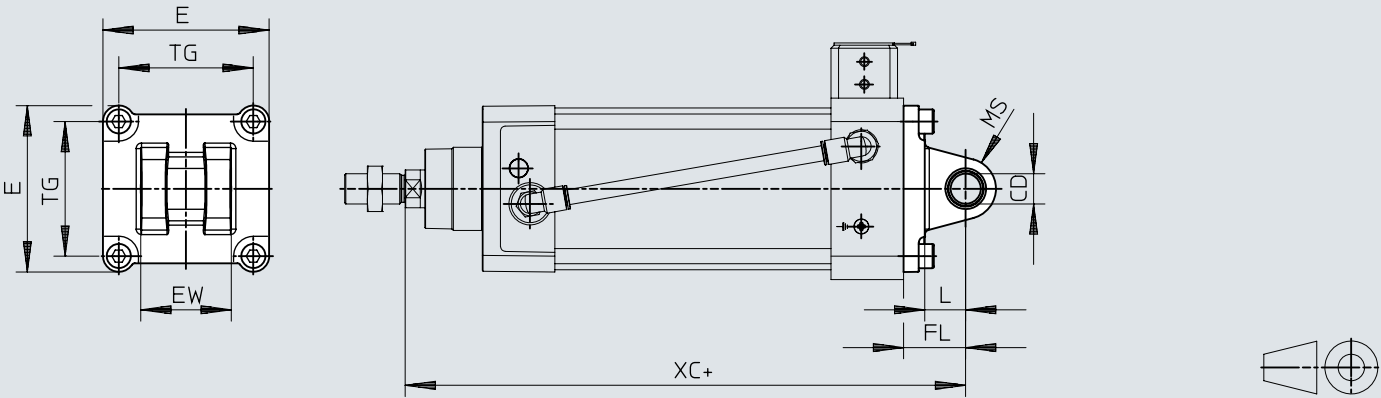
Dimensions – Swivel flange SNCL
