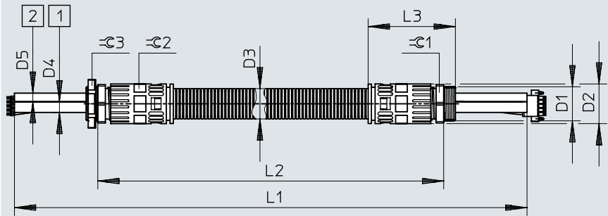
Dimensions – HNSB, 5-core
