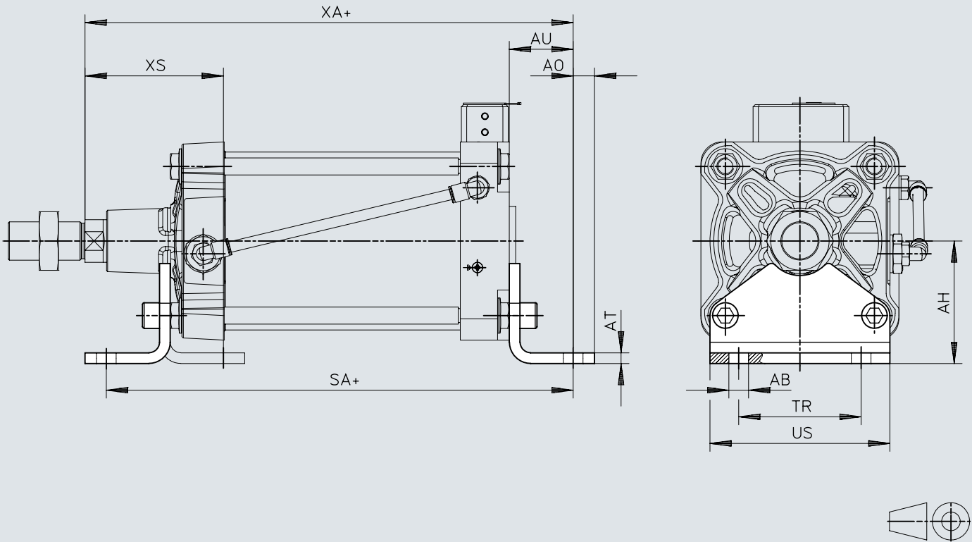
Dimensions – Foot mounting HNG, for Ø 160, 200
