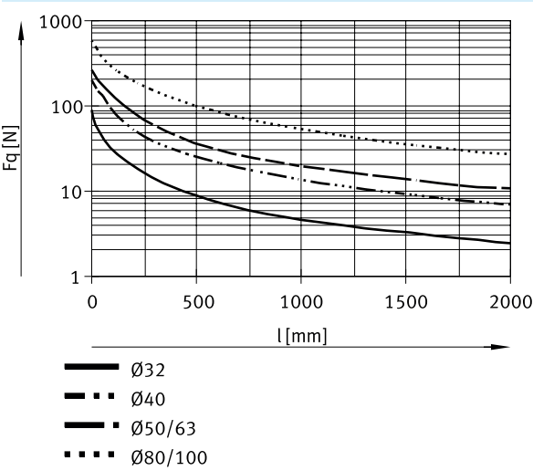
Permissible lateral force Fq as a function of stroke length l – vertical mounting
