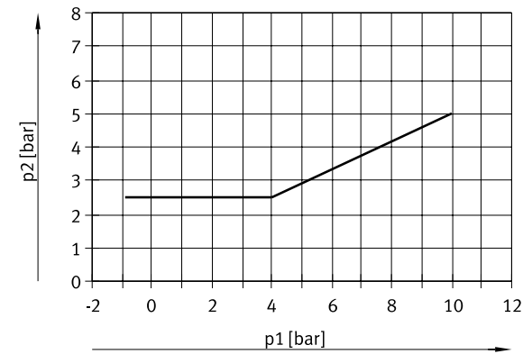
Size 20 – Pilot pressure p_2 as a function of working pressure p_1 with external pilot air supply
