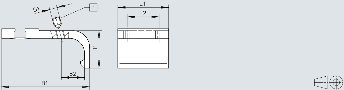
[1] Threaded pin
