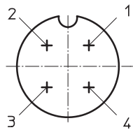
[1] 1xM12 plug, 4-pin to EN 61076-2-101
