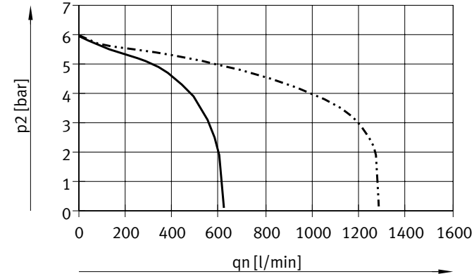
Flow rate q_n as a function of output pressure p_2 with pressure regulator plates (P regulator plate) for port 1 6 bar 10 bar
