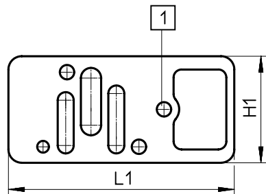
[1] With drilled hole, internal pilot air supply
