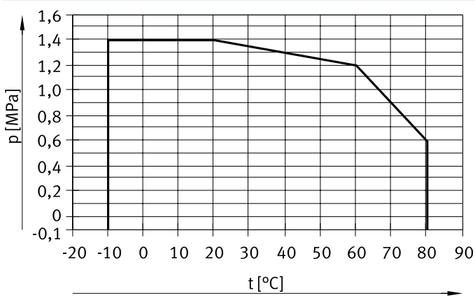
Operating pressure p as a function of temperature t (except QS-G3/4-22)
