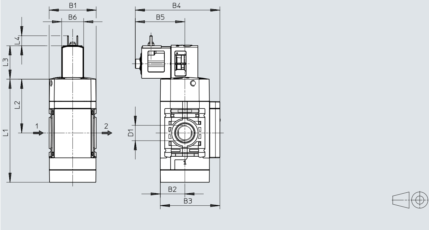
Dimensions – Basic version
