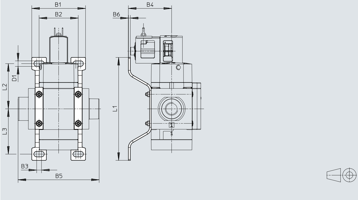
Dimensions – Wall mounting kit MS...-WPE-B (accessories)
