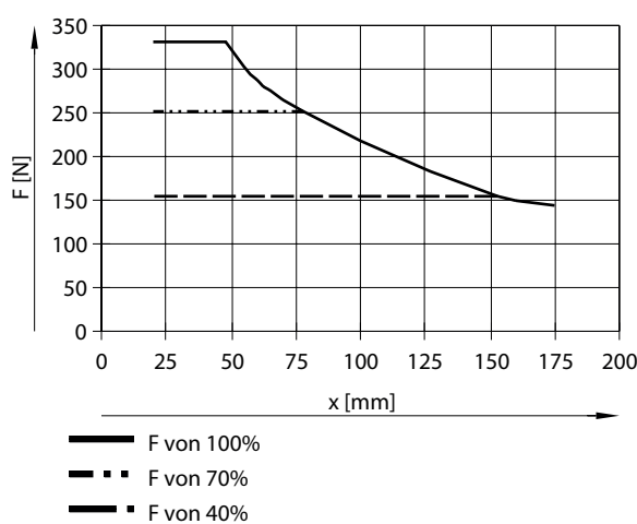
Gripping force F as a function of lever arm x for HEPP-42
