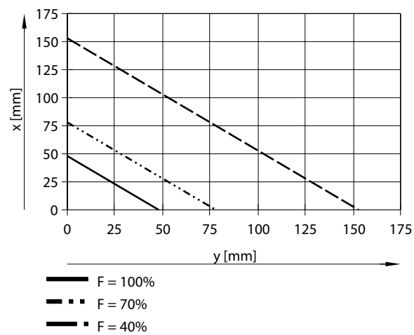
Gripping force F as a function of gripping point x/y for HEPP-42
