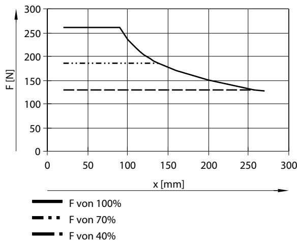
Gripping force F as a function of lever arm x for HEPP-36
