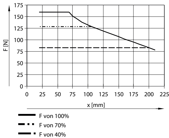
Gripping force F as a function of lever arm x for HEPP-28
