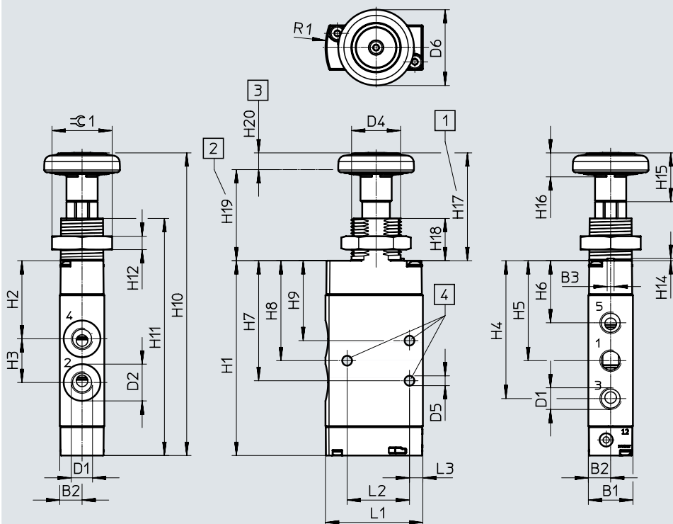
[1] Normal position [2] Actuated position [3] Valve stroke [4] Mounting holes for M4 screws
