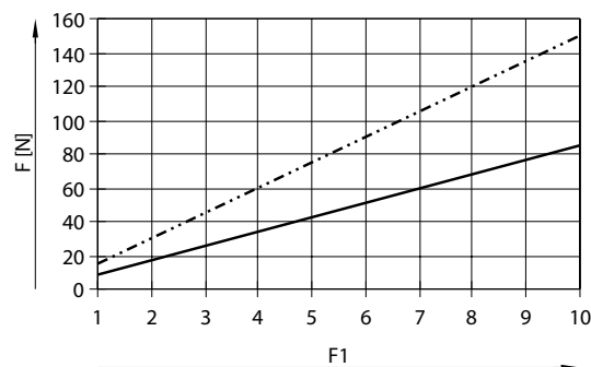
Feed force F as a function of force level F1
