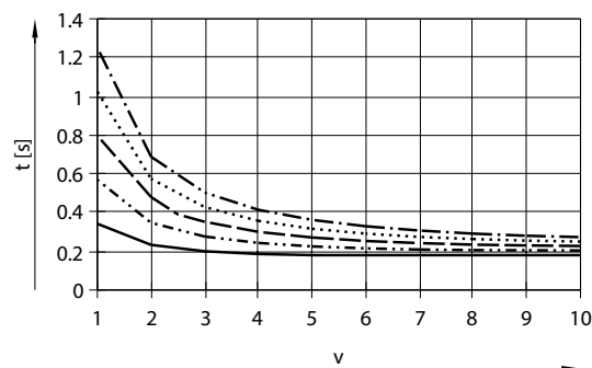
Positioning time t as a function of speed level v and stroke l EPCE-45
