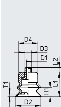
ESS-10-B
