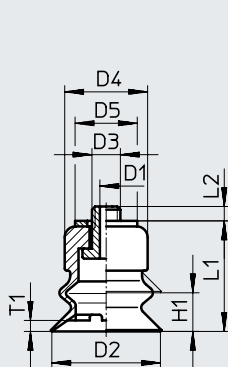
ESS-20/30-B
