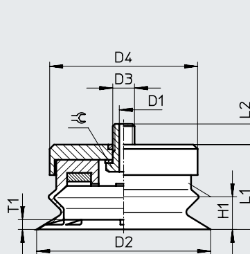
ESS-80-B
