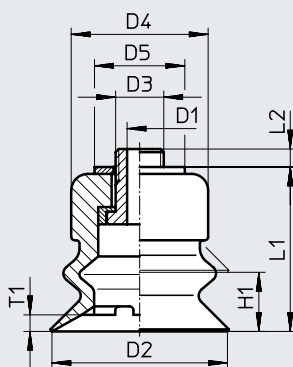
ESS-40/50-B
