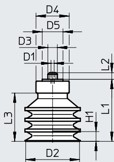
ESS-20/30-C
