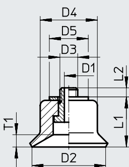
ESS-20/30-E
