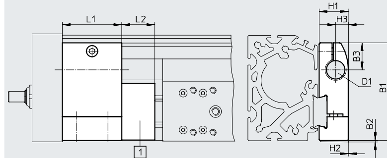
[1] Notpuffer NPE
