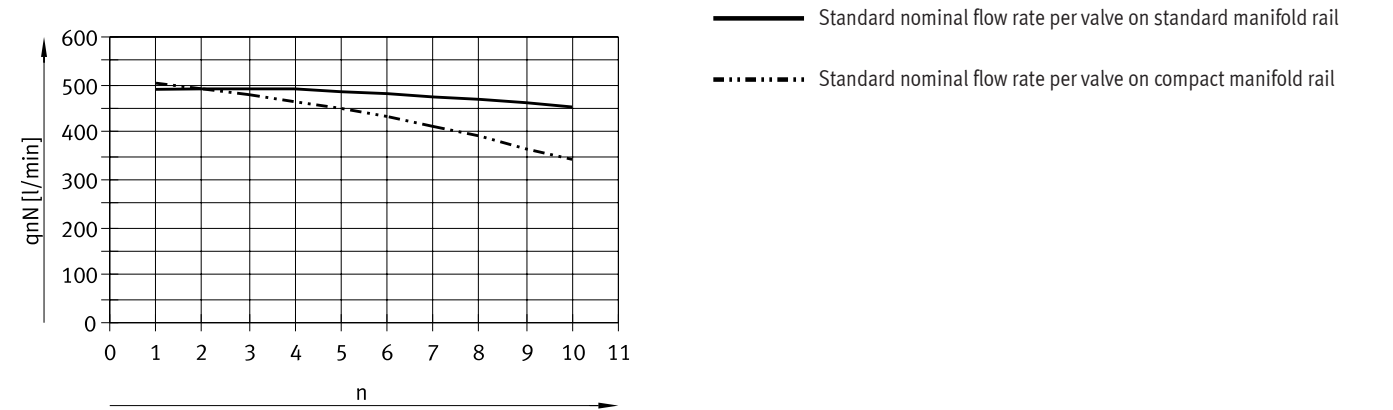
Size 20 – Standard nominal flow rate q_{nN} , with several valves n switched in parallel For 2x 3/2-way valves One valve function per valve position in open switching position
