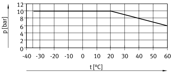
Operating pressure p as a function of temperature t
